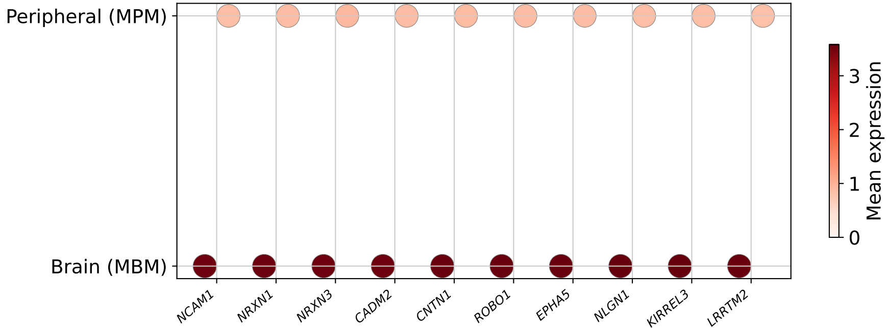
Fig 3D — Neuronal genes: MBM vs MPM (dot=% expressed, colour=mean expr)
